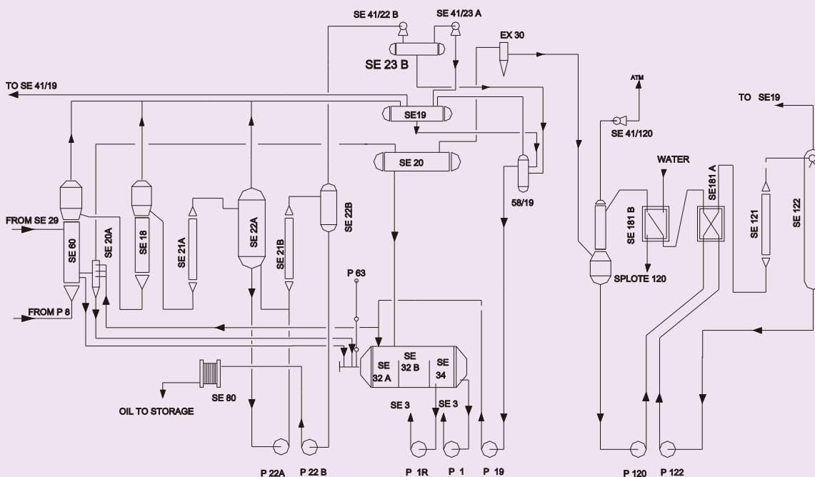
Flow Diagram - Distillation
